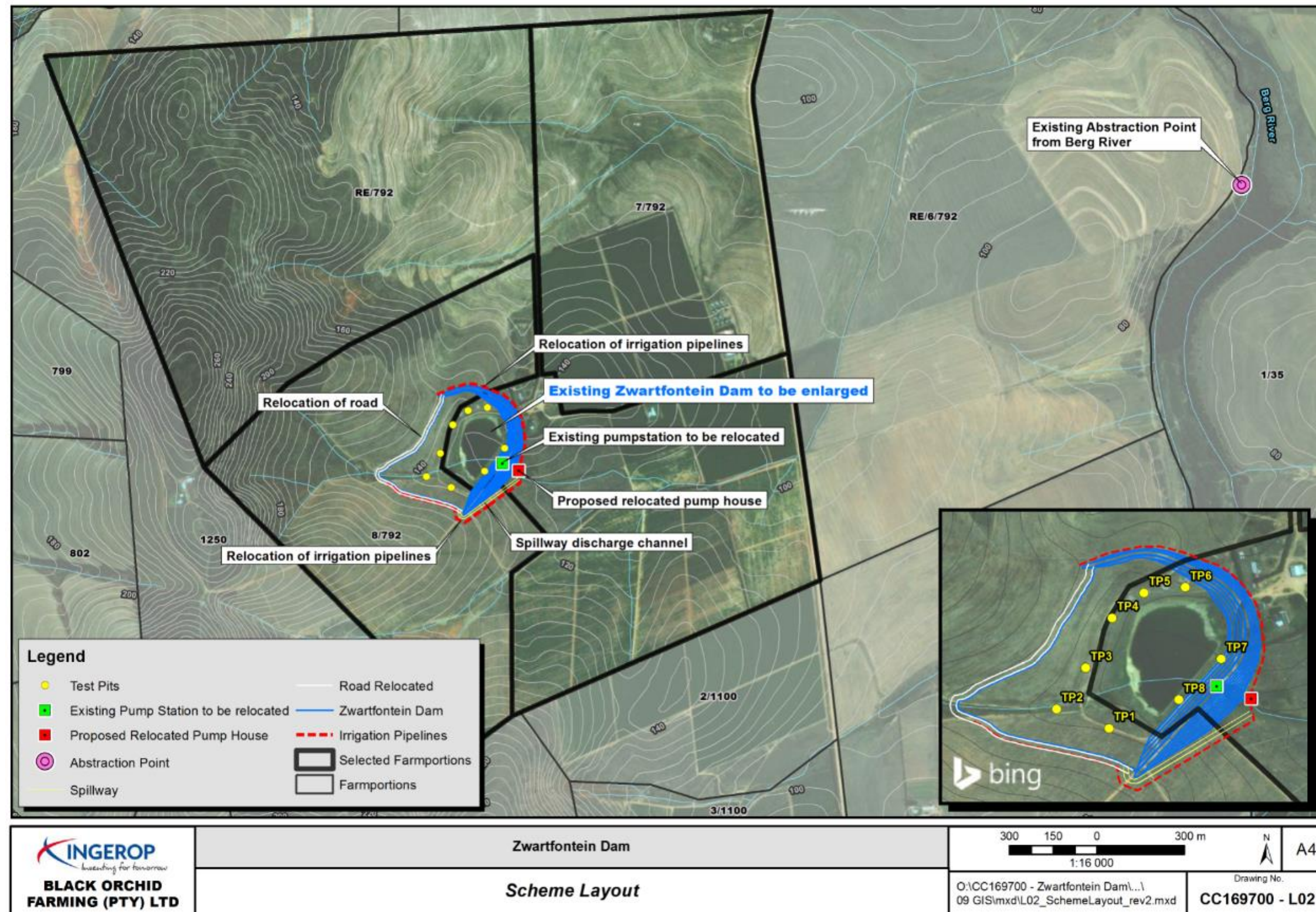
Figure 2: Proposed raised Zwartfontein Dam embankment and FSL with other listed activities
