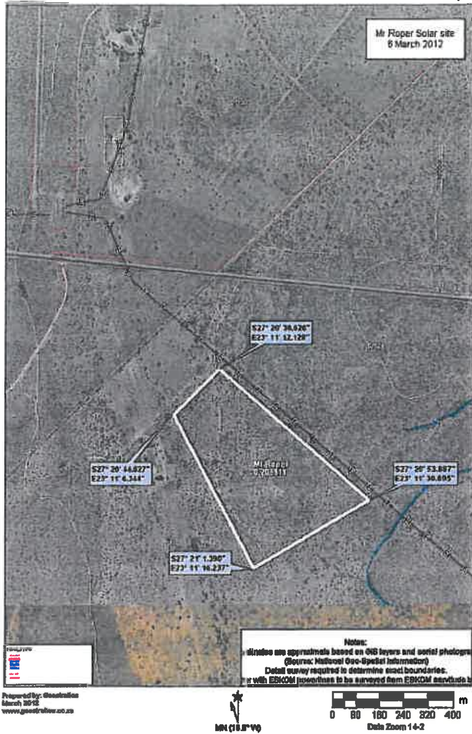
Fig. 2. Satellite image showing the study area for the Roma Energy Mount Roper Solar Plant situated on Farm 321 Mount Roper 13.2 km WNW of
