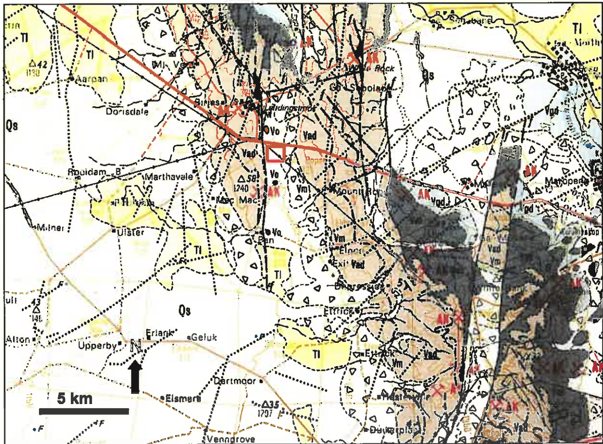
Fig. 1. Extract from 1: 250 000 geological map 2722 Kuruman (Council for Geoscience, Pretoria) showing approximate location of proposed Mount Roper Roma Solar Plant study area within a valley eroded into the northern Kurumanheuwels 27.5 km WNW of Kuruman, Northern Cape Province (small red rectangle). The study area is underlain at depth by Precambrian (Early Proterozoic) sedimentary rocks of the Daniëlskuil Formation (Asbestos Hills Subgroup, Ghaap Group, Transvaal Supergroup) (Vad). The Precambrian bedrocks of the floor of the valley are blanketed with colluvial and alluvial rock rubble (triangular symbols) as well as wind-blown sand (Qs, white). The mining symbol marked AK refers to crocidolite (asbestos) mines in the region.
