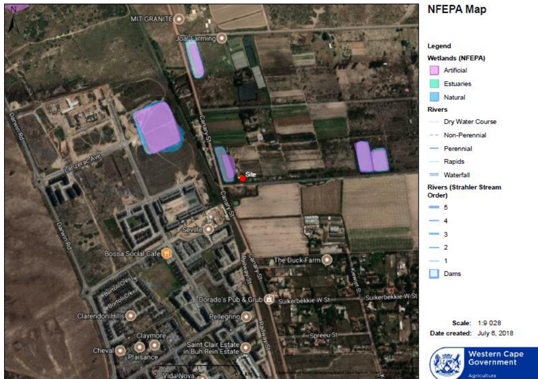
Figure 9: Cape Farm Mapper – NFEPA Map showing that the proposed site (red dot) is not located on or within 32m of any watercourse or surface water body. The site, however, is located 36m east of an artificial wetland (dam).
