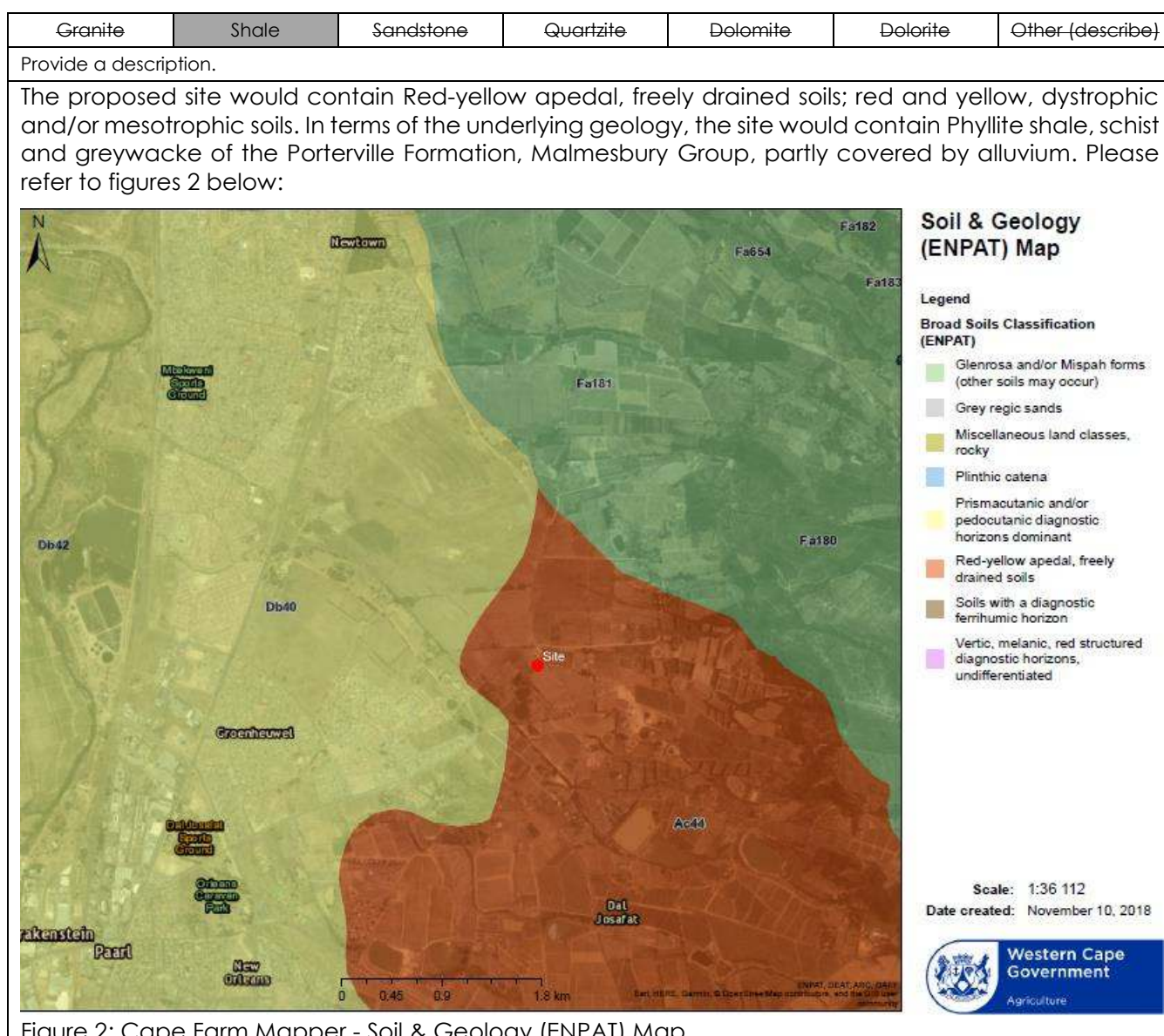
Figure 2: Cape Farm Mapper - Soil & Geology (ENPAT) Map.
