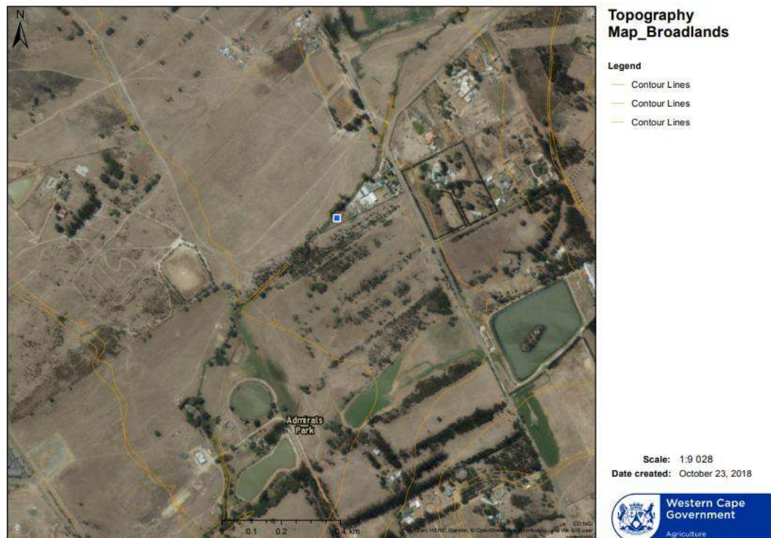
Figure 5: Topography map
