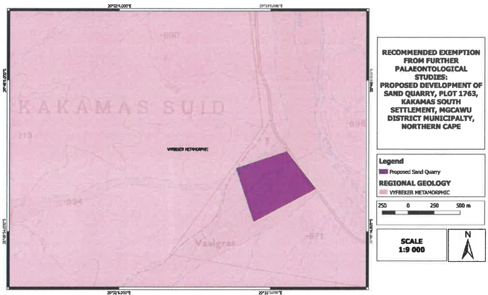
Figure 3: The surface geology of the proposed sand quarry on Plot 1763, Kakamas South Settlement, in the Kall Garib Local Municipality, Northern Cape. The proposed development is entirely underlain by the Vrybeker Metamorphic Suite of the Namaqua-Natal Province. Map drawn QGIS Desktop 2.18.18.
