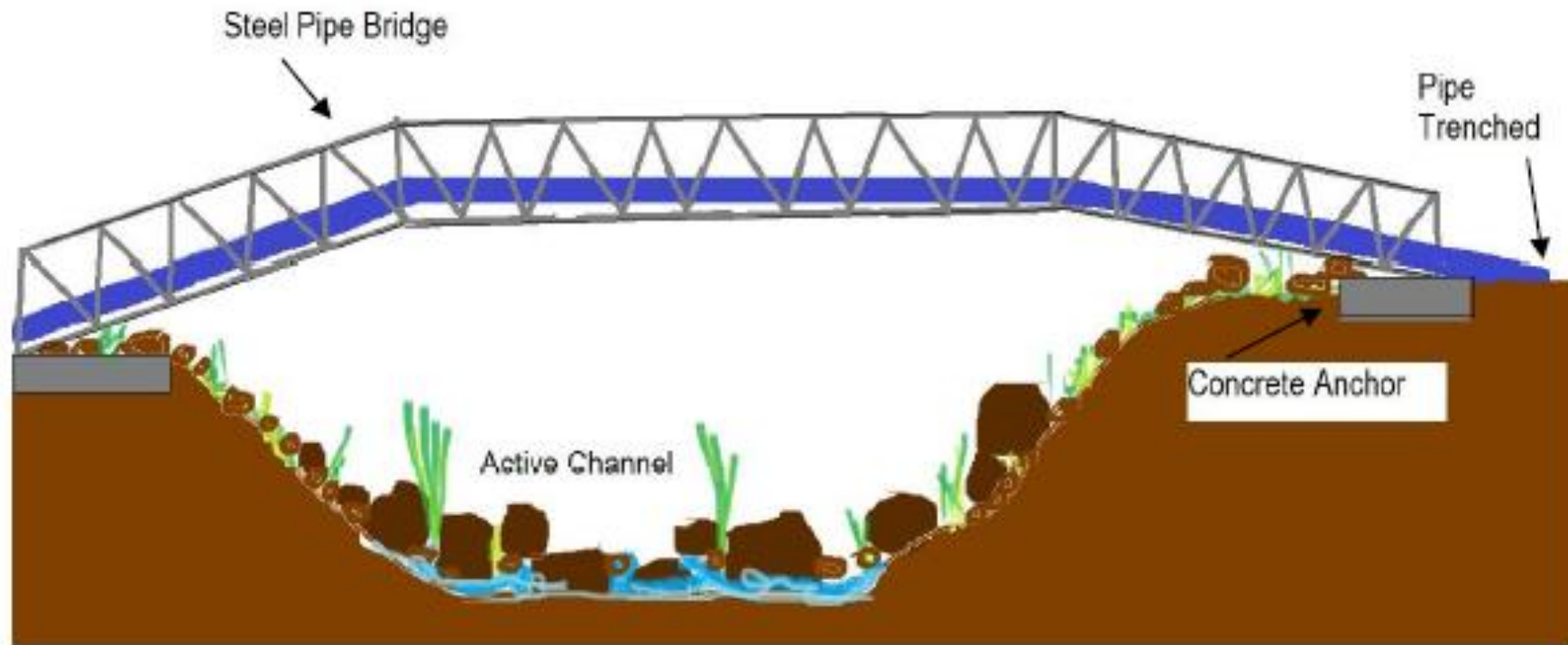
Figure 1: Conceptual diagram from the River Rehabilitation & Maintenance Management Plan (RRMMP) showing a steel pipe bridge spanning the active channel of the river, anchored on either embankment. The proposed pipeline is initiated in dark blue and will be trenched leading up to and following from the pipe bridge.
