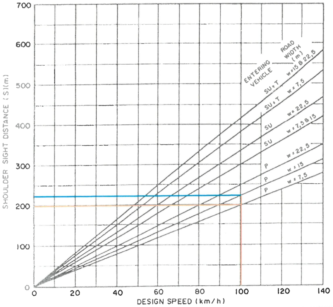
SHOULDER SIGHT DISTANCE FOR STOP CONDITION
