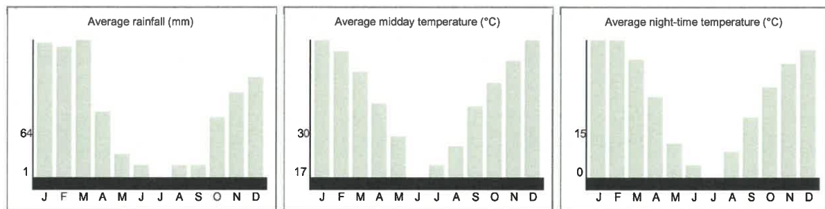
Figure 2 Dealesville Climate
