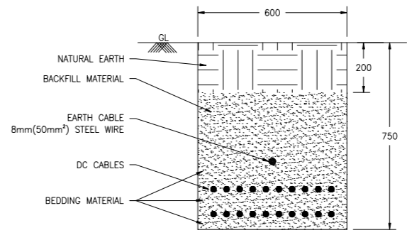
TYPICAL SECTION OF DC TRENCH CROSSINGS 600mm WIDE SCALE 1:2
