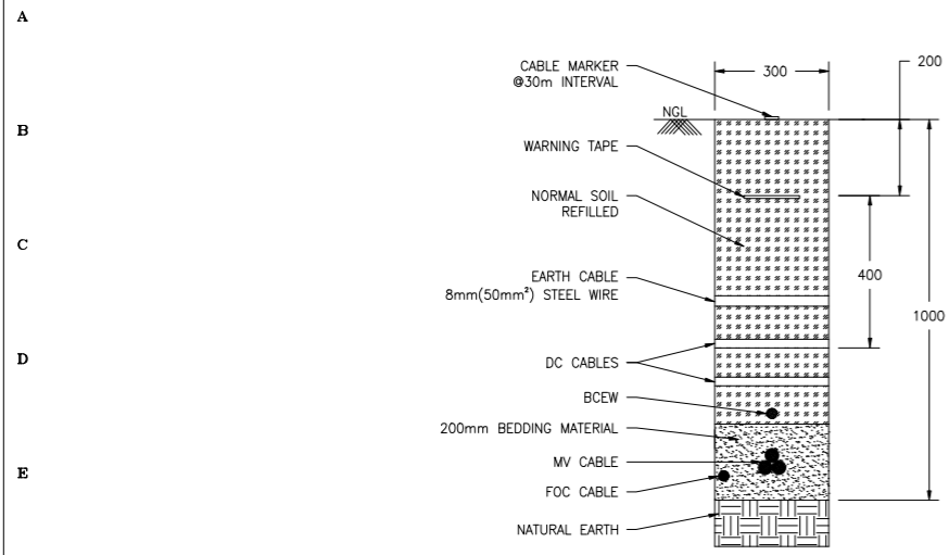
TYPICAL SECTION OF AC TRENCH CROSSINGS 300mm WIDE SCALE 1:2
