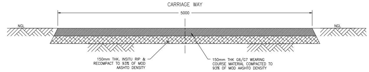
5.0m WIDE MAIN ROAD TYPICAL CROSS SECTION - TYPE 1
