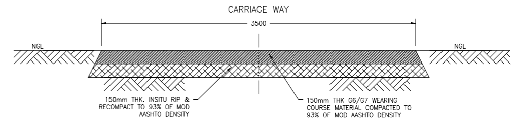
3.5m WIDE ROAD TYPICAL CROSS SECTION - TYPE 2
