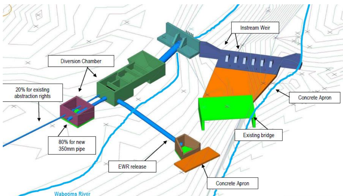
Figure 5: 3D drawing of Water Structure Alt 1: new weir, water diversion chamber & pipelines
