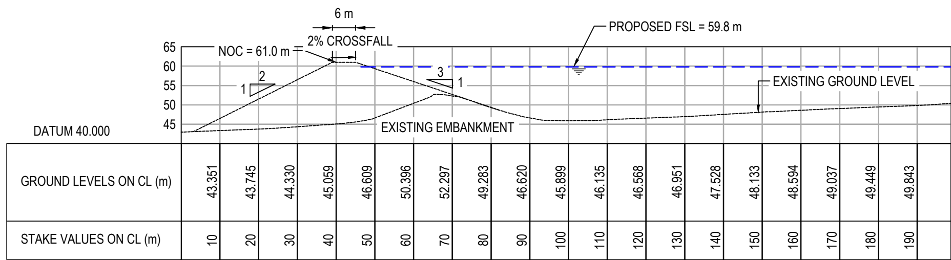
SECTION THROUGH CREST CENTRELINES: RAISING OF DAM FROM 0.000 TO 198.764 SCALE 1:1000
