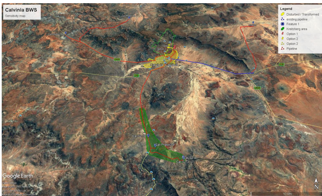
Figure 7: Calvinia BWS sensitivity map: The Kreitzberg area and the Akkerendam NR in green, the disturbed urban edge of Calvinia in yellow.
