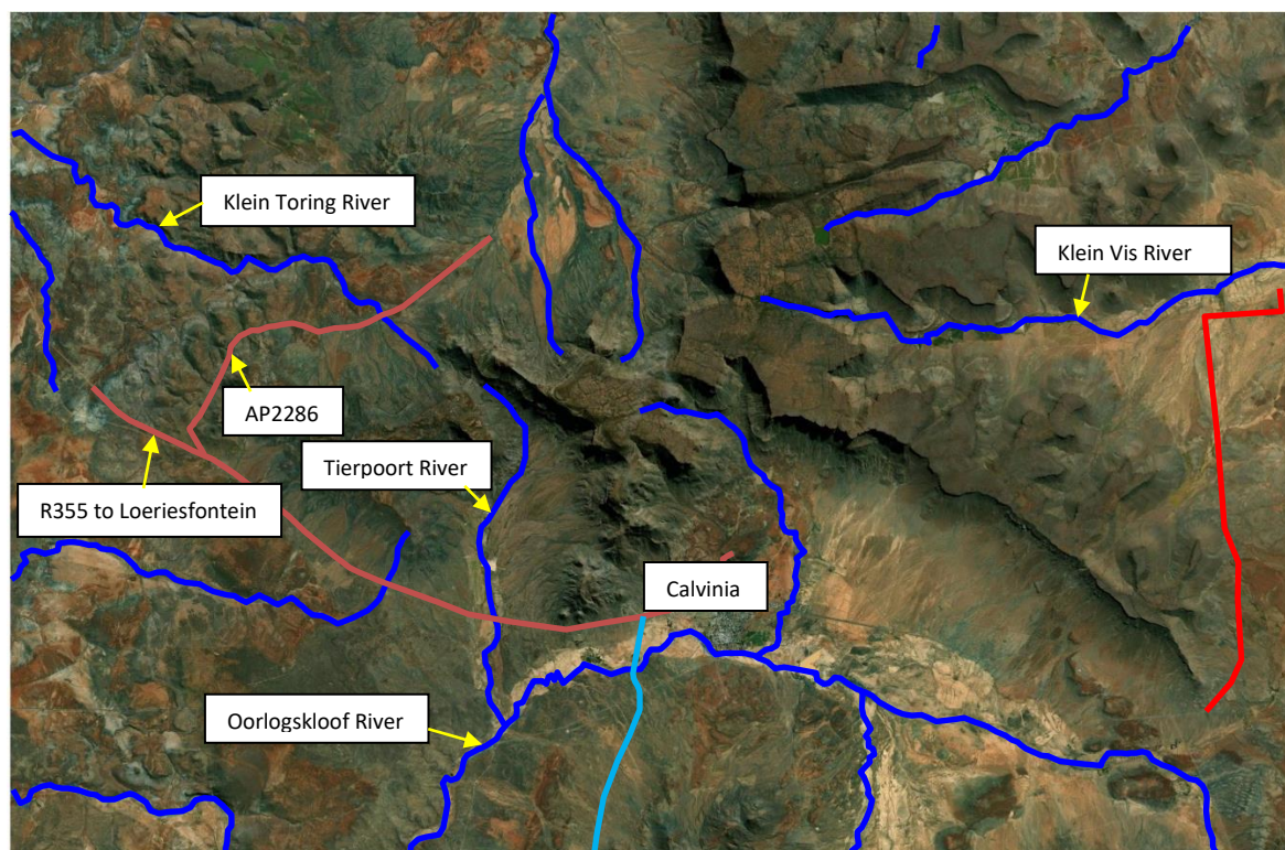
Figure 6: Google Earth showing major watercourses north of Calvinia
