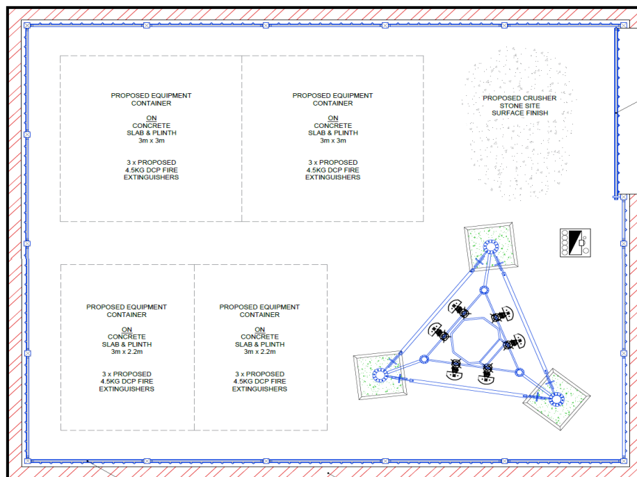
Figure 2. The layout of the proposed development of a 35m high telecommunication mast on Portion 22 of Farm 22, Zouterivier. Source: CTC Operations.
