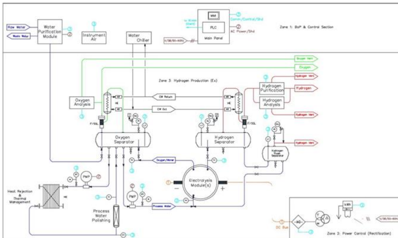
FIGURE 2: Hydrogen proton exchange membrane electrolysis simplified process flow diagram
