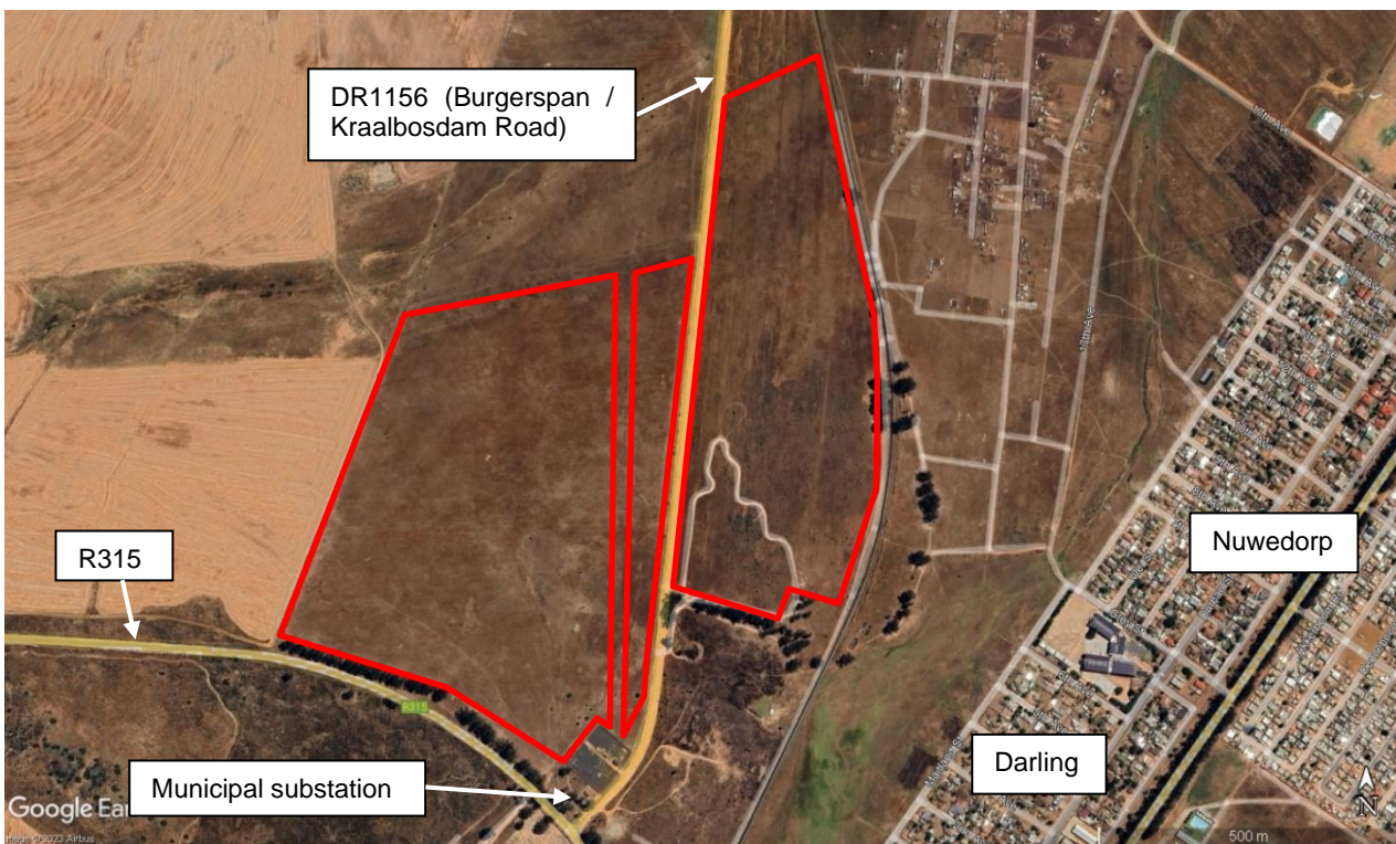
Figure 2: Google Earth image of the proposed solar PV site (red polygons).
