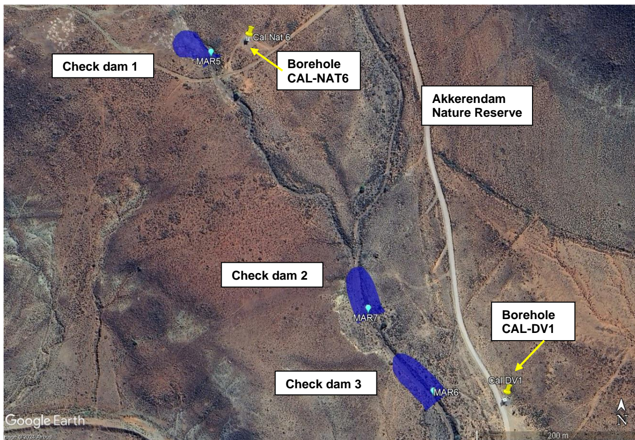
Figure 8: Location of the Check Dams at infiltration boreholes MAR 5, 6 and 7.
