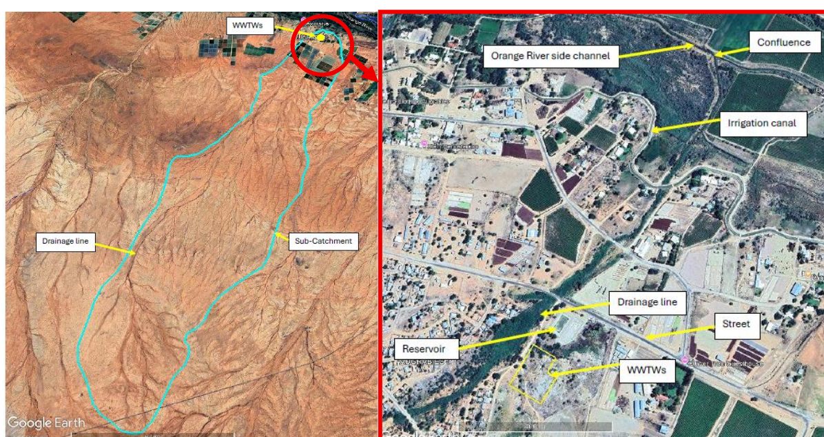
Figure 3: View of sub-catchments as well as drainage lines overlapping the proposed site
