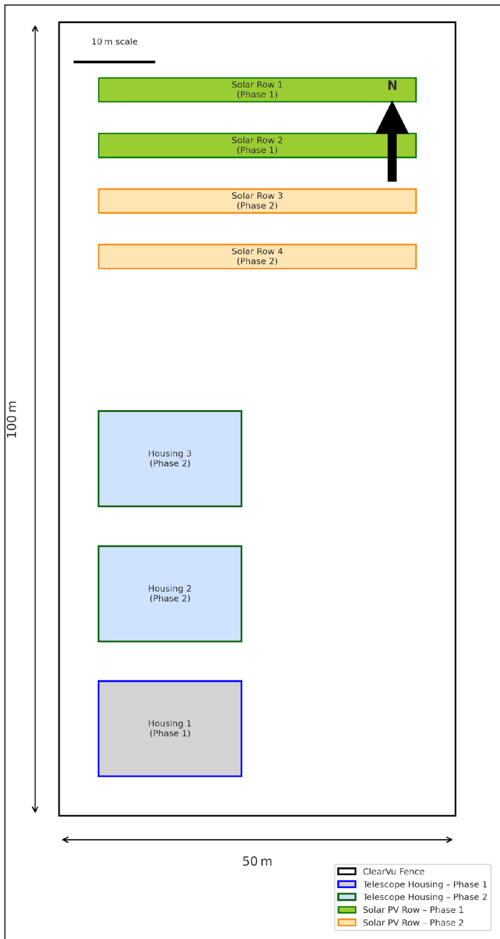
Figure 1: ZuluAlpha site plan layout for three such compounds: Phase 1 (grey/green) and Phase 2 (blue/orange)
