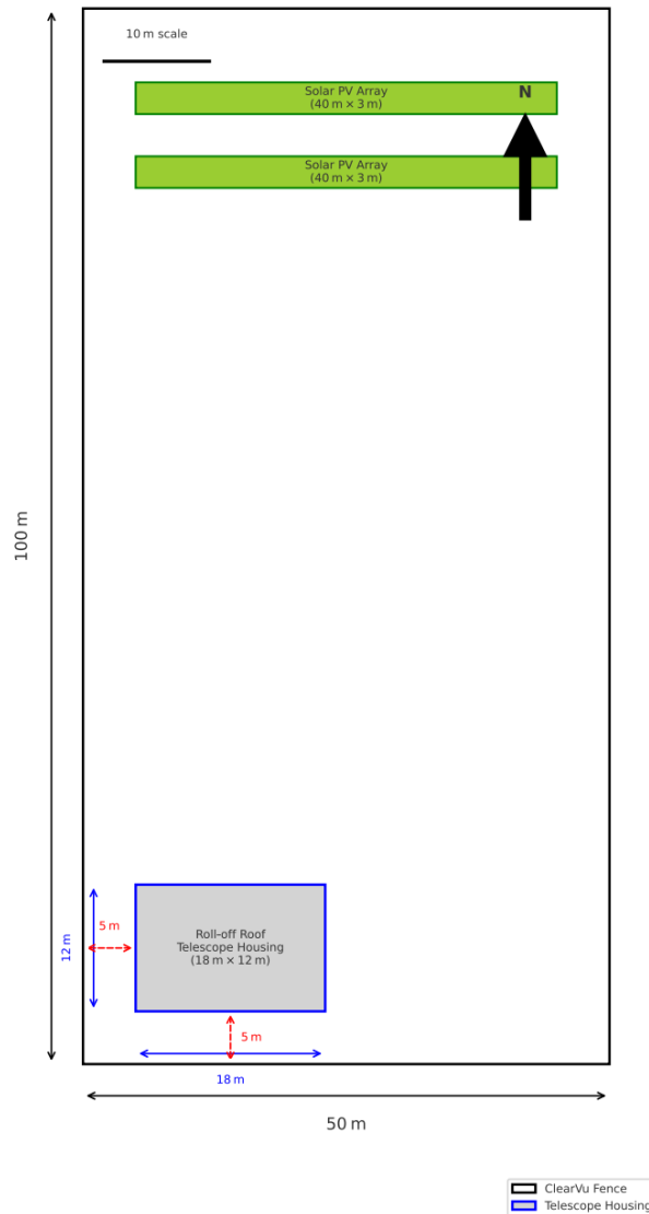
Figure 3: Layout for Phase 1 of the ZuluAlpha telescope and boundary fence.
