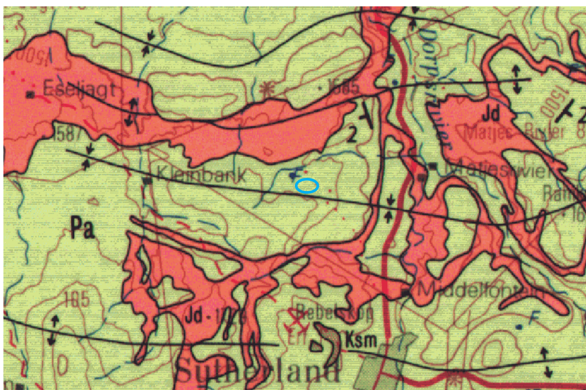
Figure 4: Geological map of the area around the ZuluAlpha telescope site, as indicated within the blue outline. Abbreviations of the rock types are explained in Table 2. Map enlarged from the Geological Survey 1: 250 000 map 3220 Sutherland.
